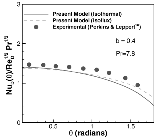
Fig. 9 Local Nusselt number for two thermal boundary conditions.
