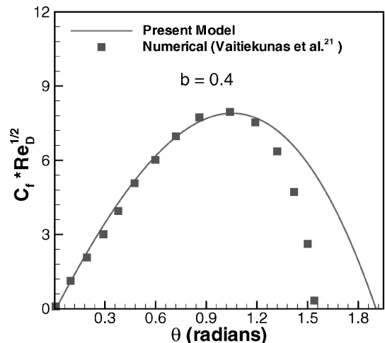
Fig. 5 Distribution of dimensionless shear stress for given blockage ratio.
